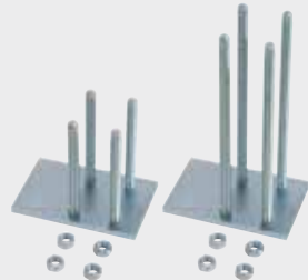
Pair of fixing plates and nuts for application on metal doors with long screws: - 50 mm (item 4008.0757) (standard accessory) - 95 mm (item 4008.0780) (accessory always on request)
